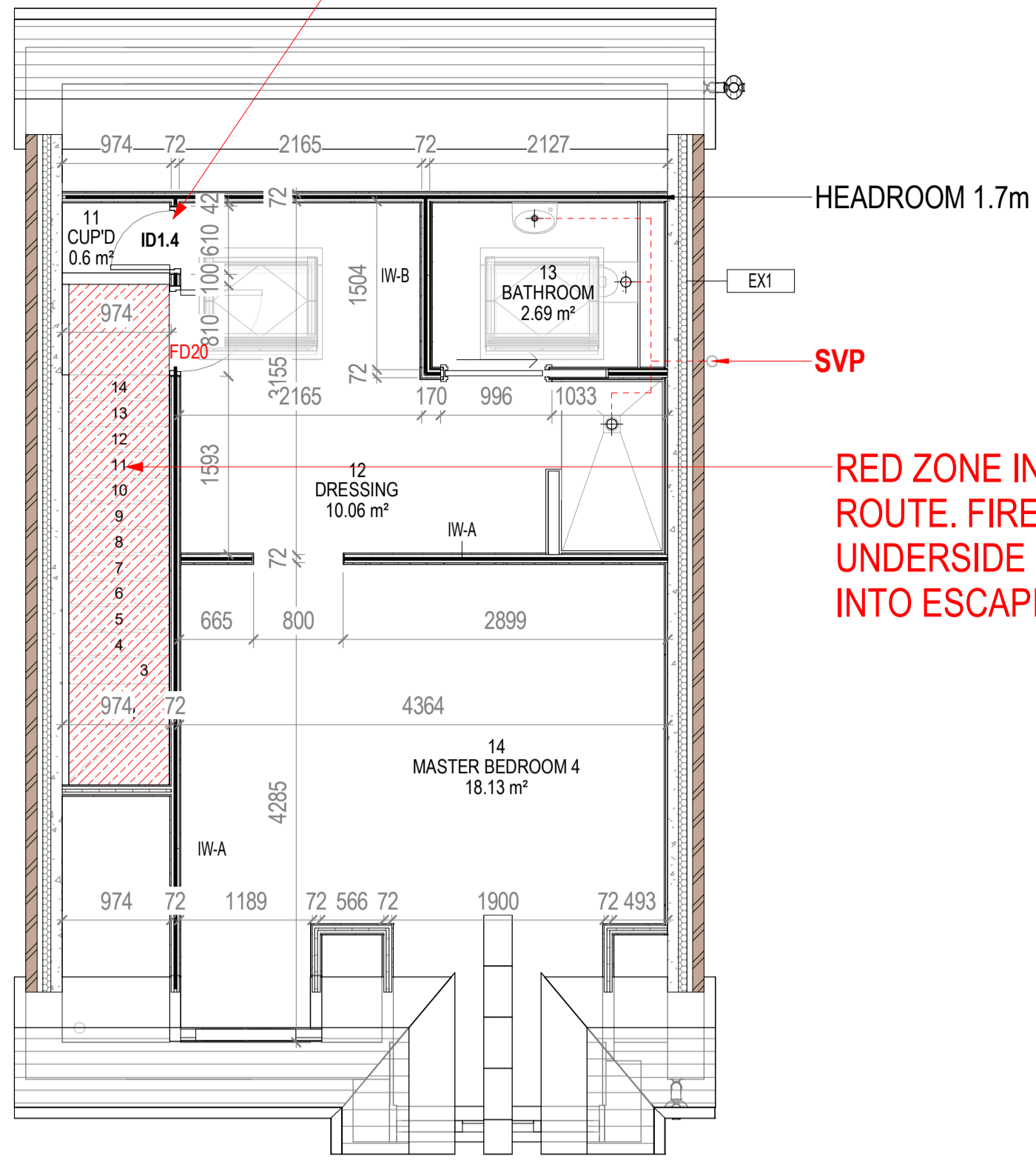
Level 02_Setting Out
