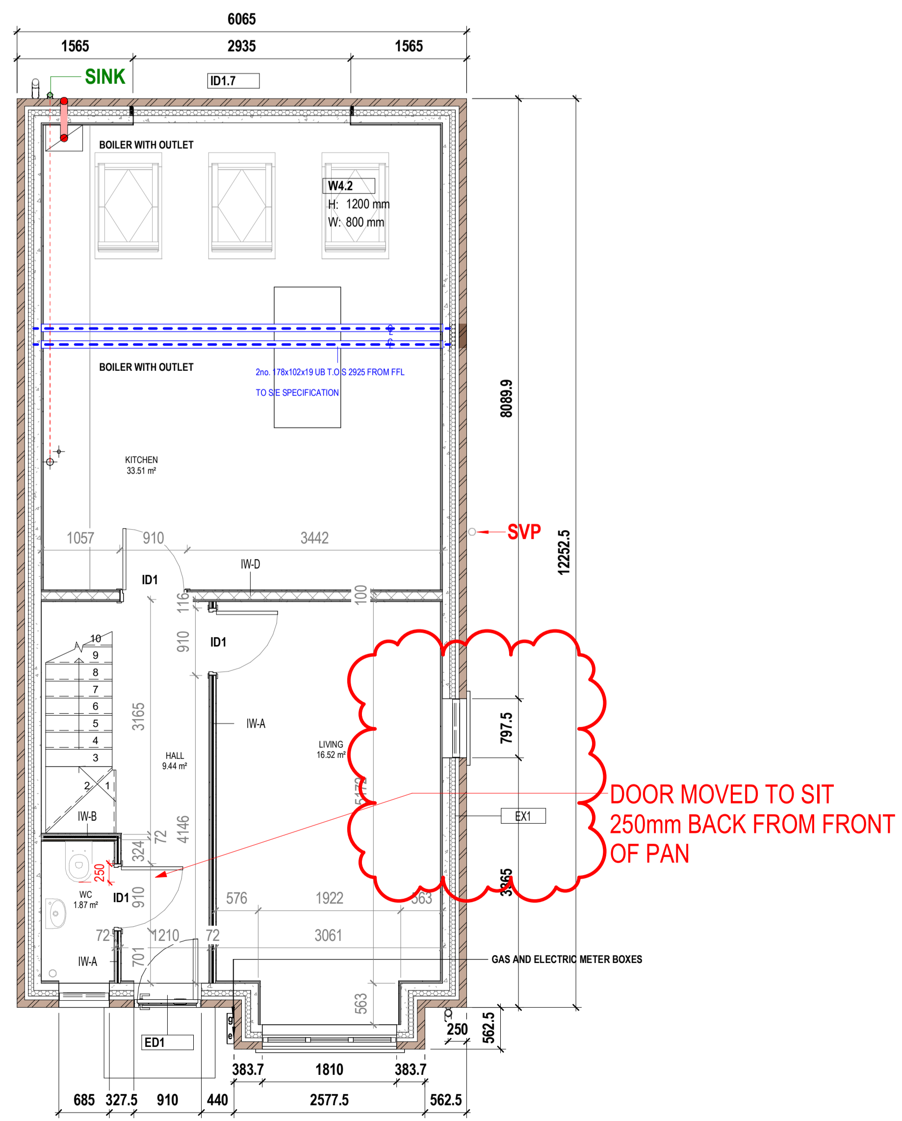
1 Level 00_Setting Out - DETACHED
