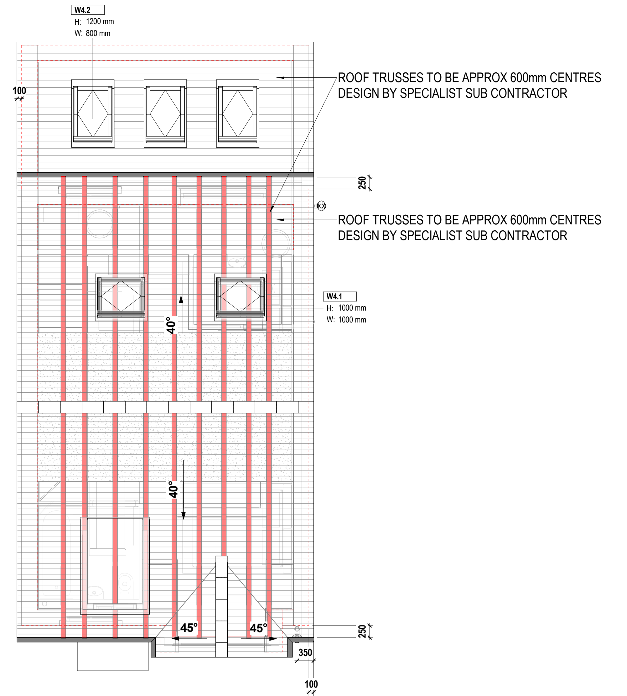
4 Roof_Setting Out - Detached
