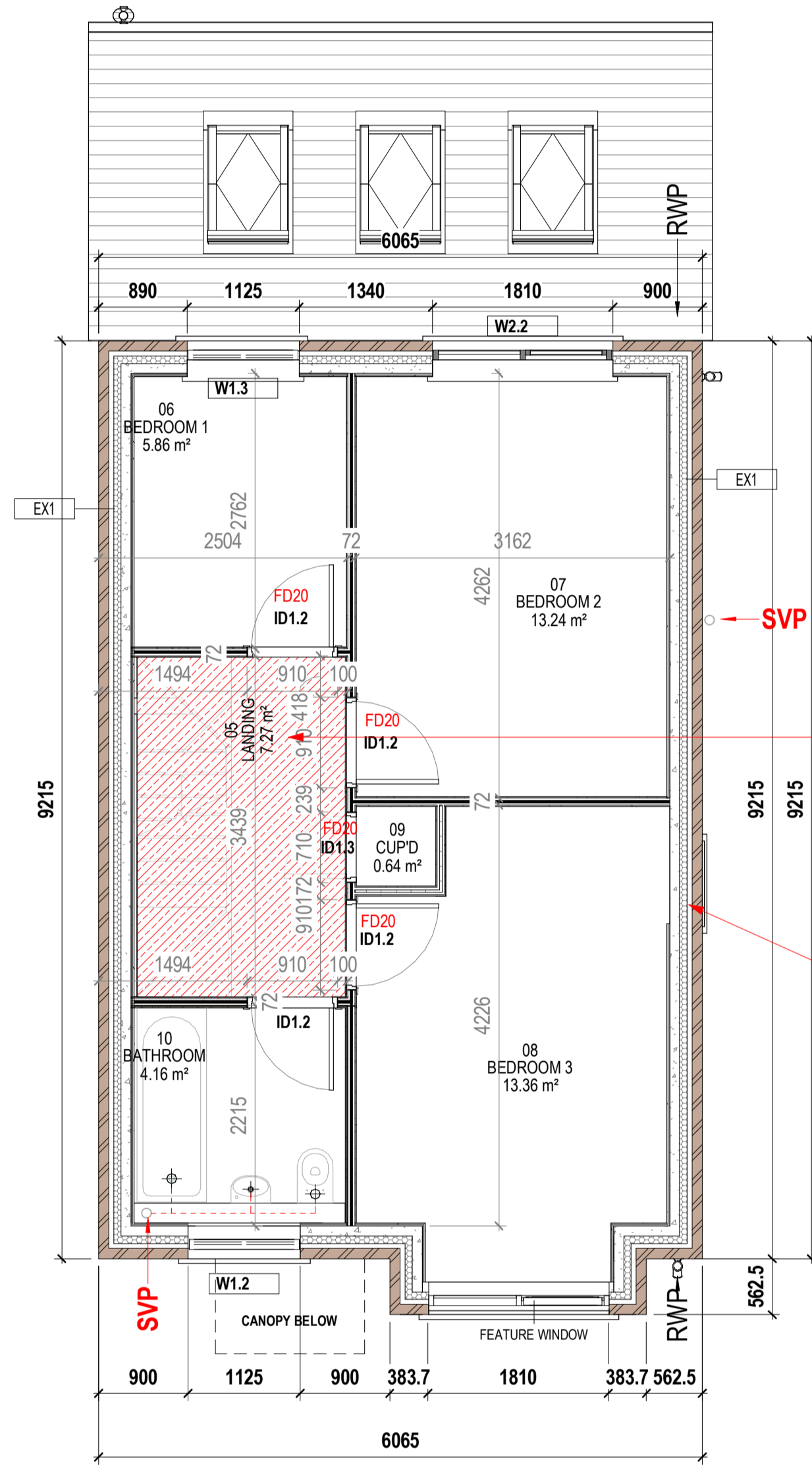
Level 01_Setting Out
