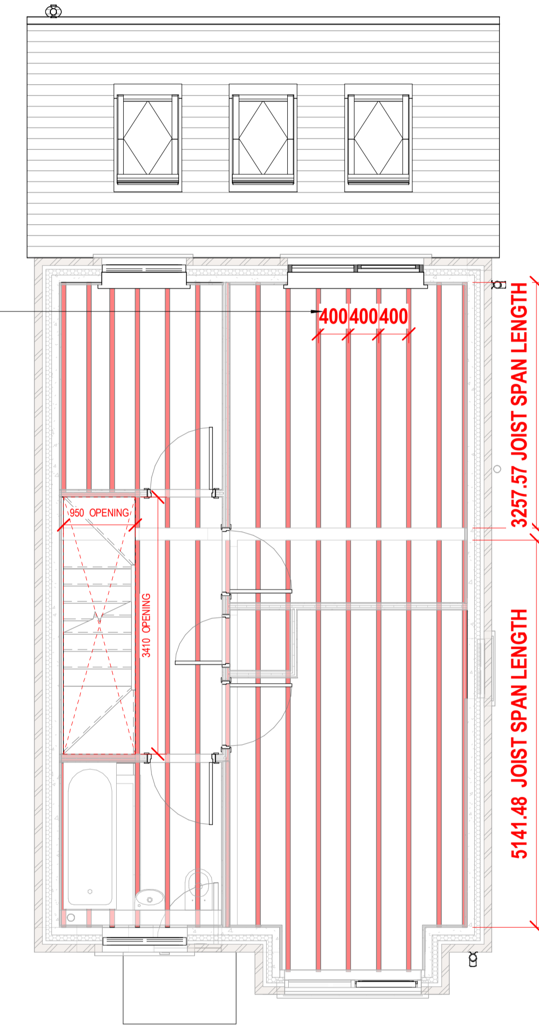
Level 01_FLOOR JOISTS
